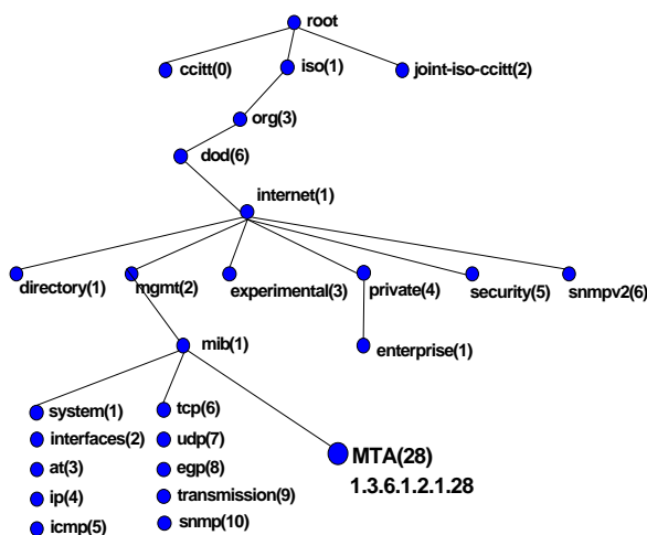
Figure 1. MTA MIB in the SNMP OID Tree
