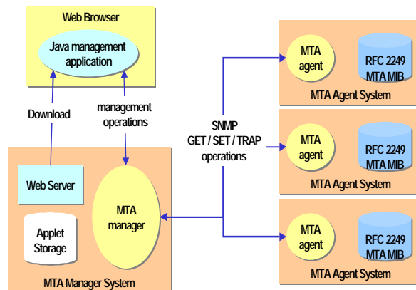
Figure 2. Design Architecture of the Proposed Mail Server Management System
