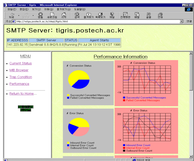
Figure 5. Performance View Window
