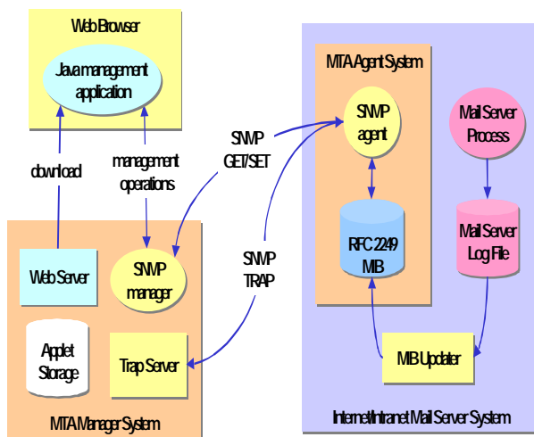
Figure 3. Implementation Architecture of Proposed Mail Server Management System
